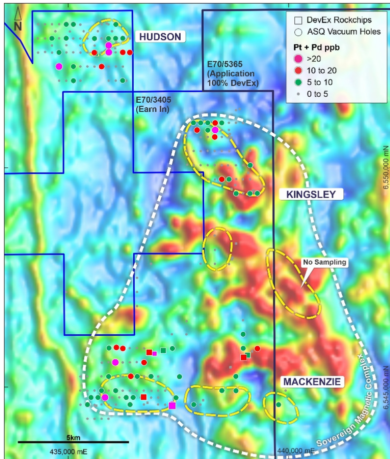
Airborne magnetic (RTP) and new AEM targets (yellow outline) with Pd + Pt analysis of pulps from ASQ Bauxite Drilling and Company rock chip (duricrust) sampling.
