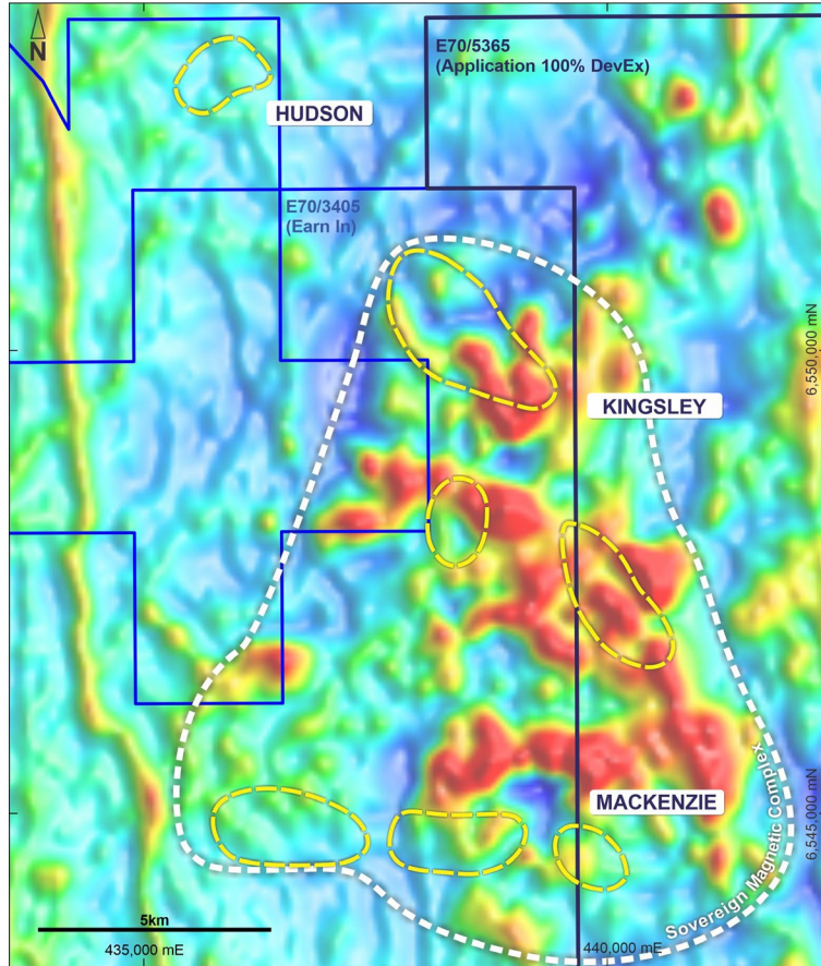
Airborne magnetic (RTP) and new AEM targets (yellow outline)
