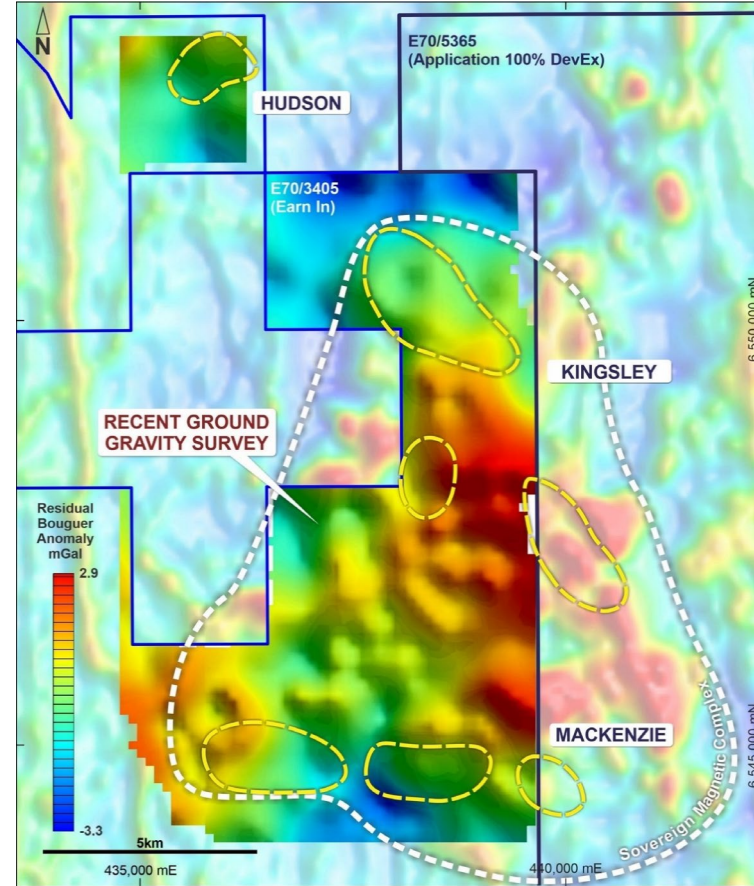
Ground gravity (Residual Bouguer) and new AEM targets (yellow outline)
